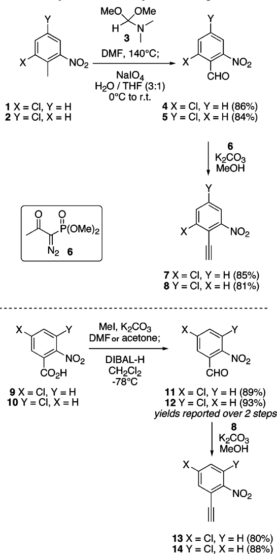
SCHEME 1. Synthesis of Acetylenic Dienophiles
