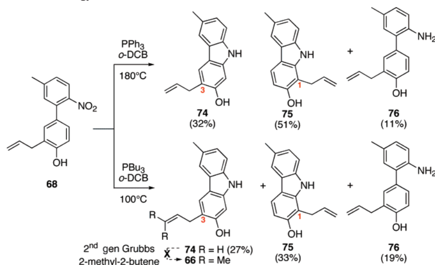
SCHEME 10. Total Synthesis of Siamenol
