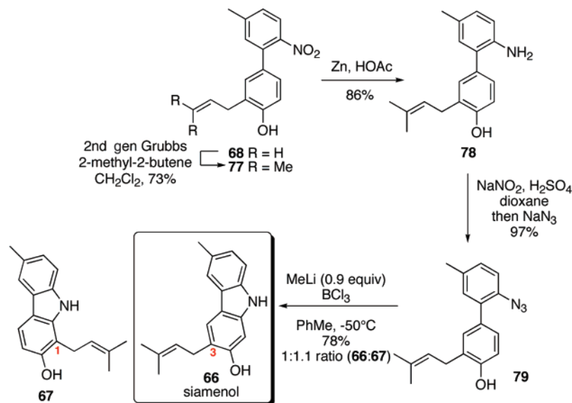
SCHEME 10. Total Synthesis of Siamenol
